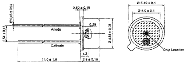
TO-46C • TL CAN
