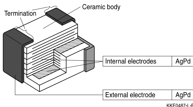
Multilayer varistor: Structure of silver-palladium termination
