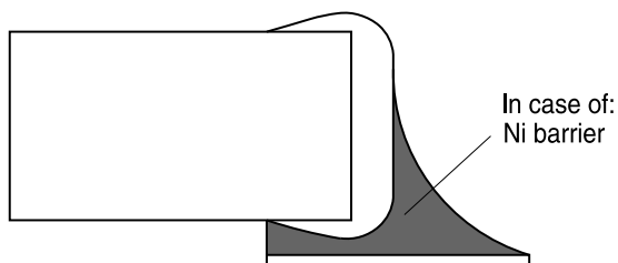
Good solder joint
