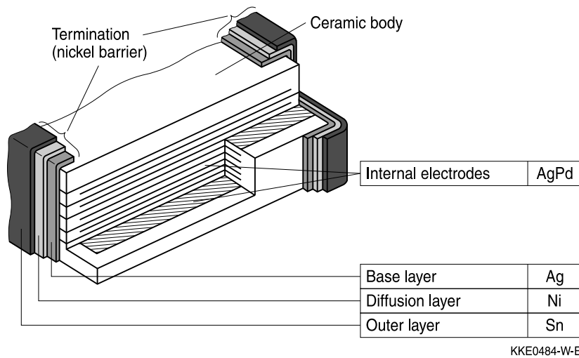
Multilayer CTVS: Structure of nickel barrier termination
