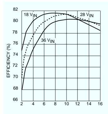
Output Power (Watts) Representative of all models MTO2815T Efficiency
