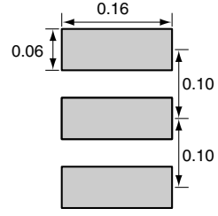
RECOMMENDED FOOTPRINT
