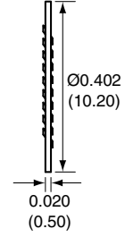
WASHER
