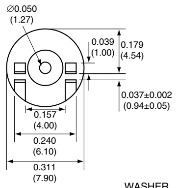
WASHER
