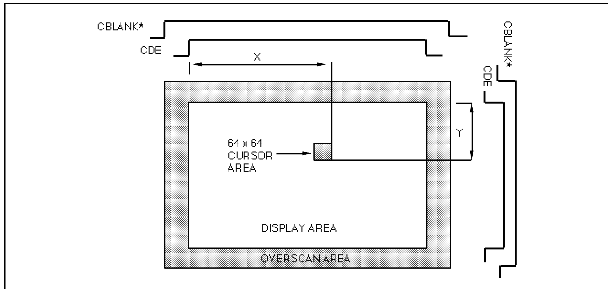
Figure 6. Cursor Positioning.
