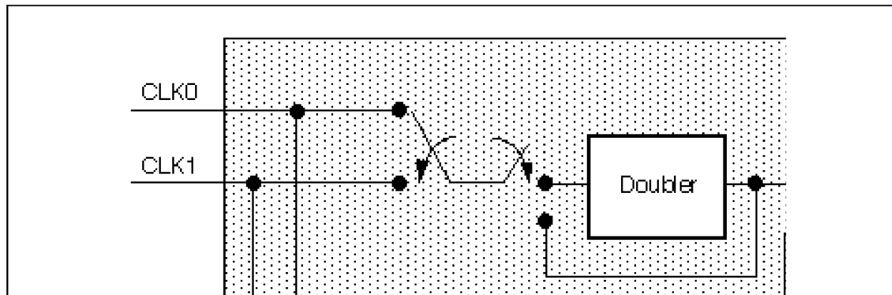
Figure 2. Bt485A Clocking.
