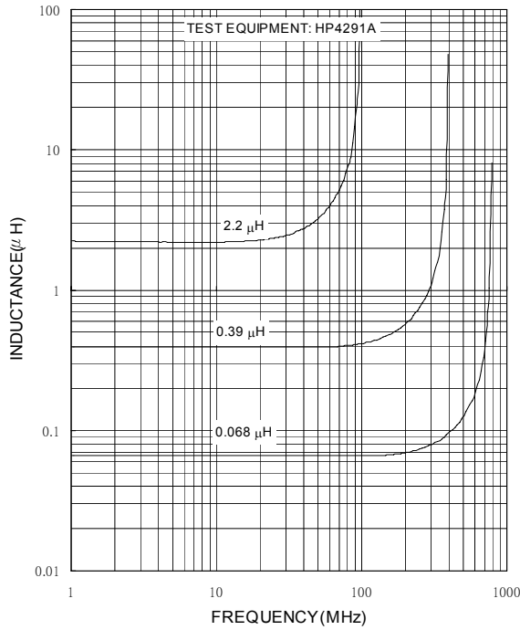
Inductance VS. Frequency
