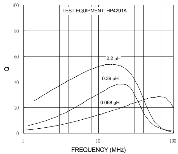
Q VS. Frequency
