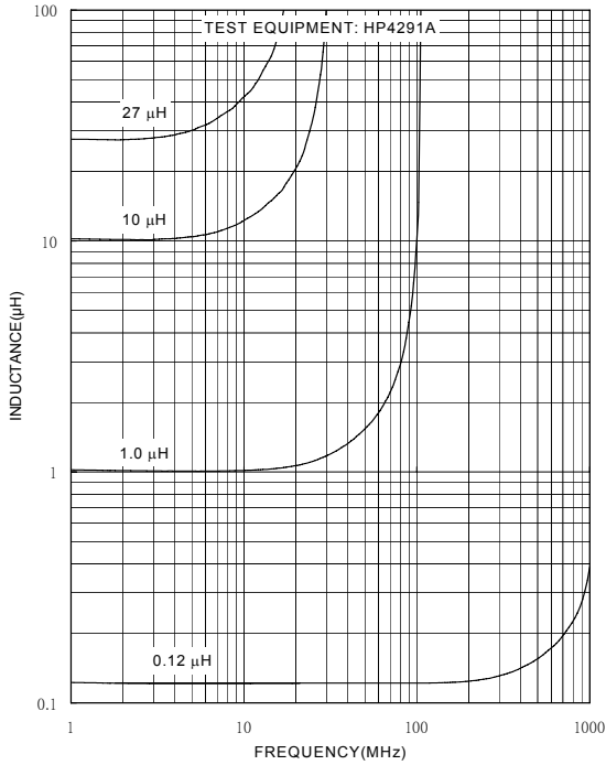
Inductance VS. Frequency
