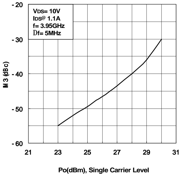
IM3 vs. Output Power Characteristics
