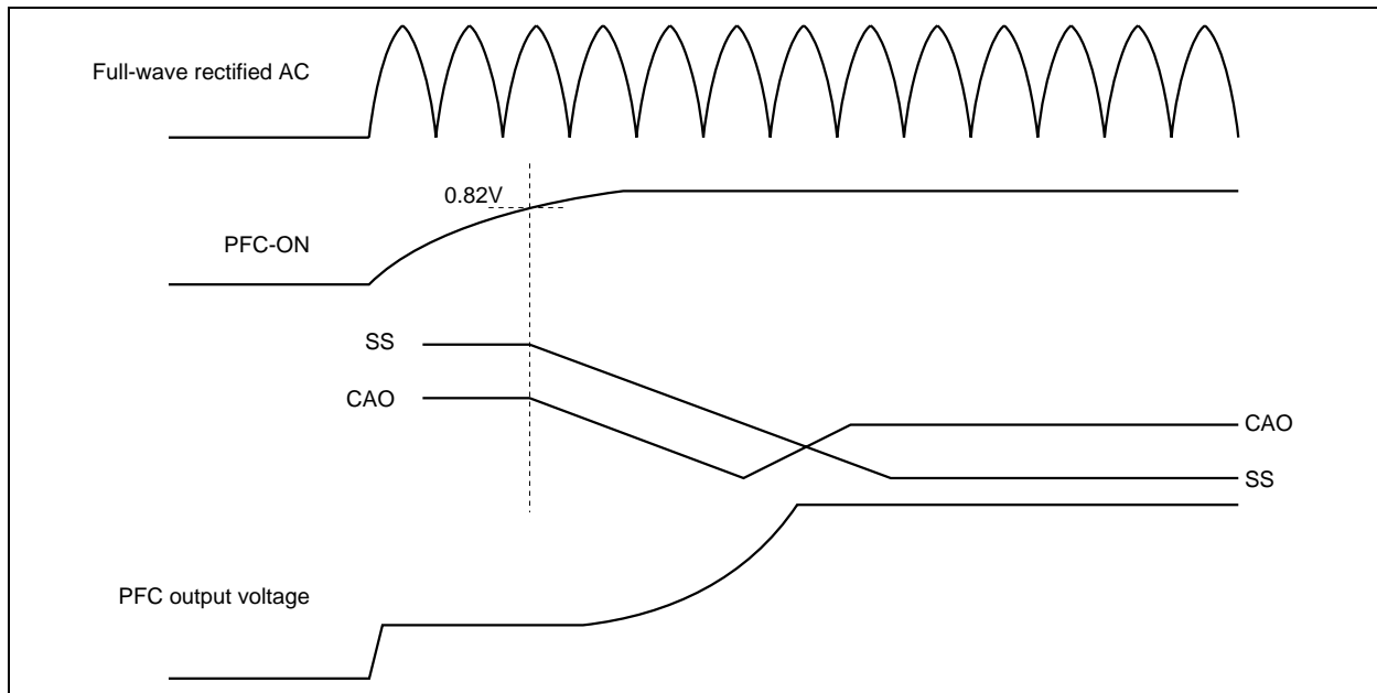
Figure 5 Waveform in Operations in Startup
