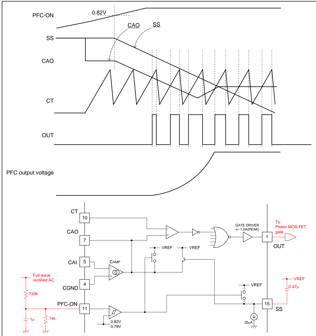
Figure 3 Soft-Start Operation Waveform
