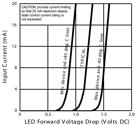
Figure 3. Input Characteristics (Current Controlled)
