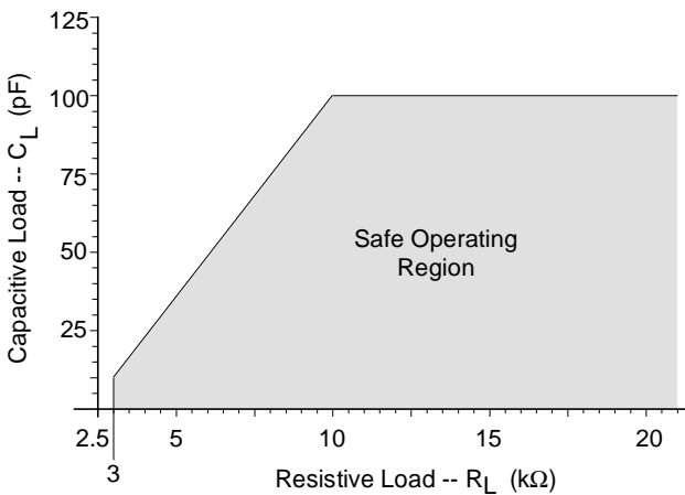
Figure 18. Maximum Loading
