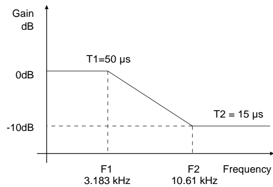
Figure 39. De-Emphasis Curve
