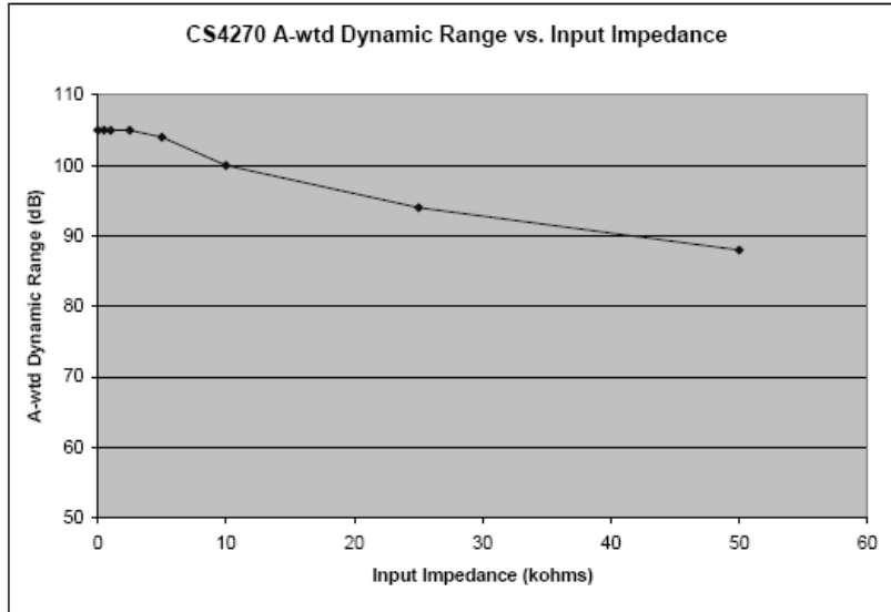
Figure 17. A/D Dynamic Range vrs. Input Source Resistance
