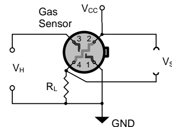
Figure 3: Measurement circuit for O 3 detection.
