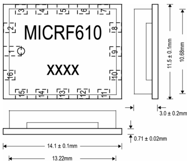
Figure 15. Package Dimensions
