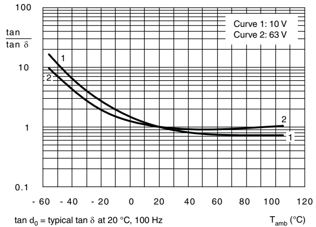
Fig.6 Typical multiplier of dissipation factor (tan d) as a function of ambient temperatures
