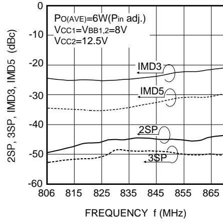
SUPRIUS, IMD VS. FREQUENCY
