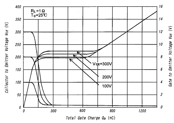
Fig. 4 Charge vs. Collector to Emitter Voltage (Typical)
