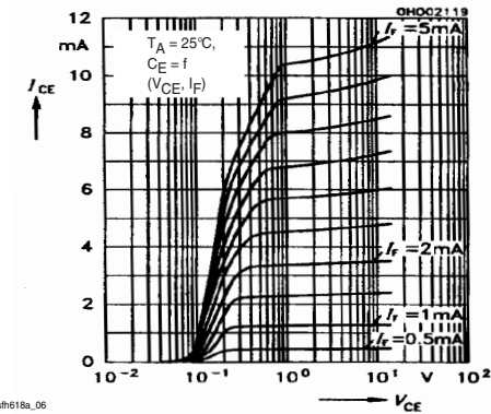
Fig. 8 Output Characteristics
