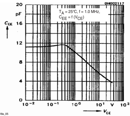
Fig. 7 Transistor Capacitance
