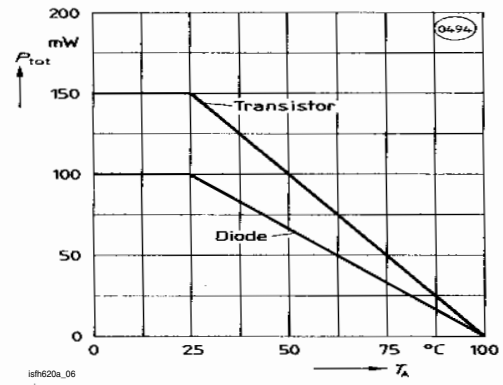
Fig. 7 Permissible Power Dissipation vs. Ambient Temperature
