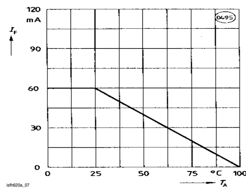
Fig. 8 Permissible Diode Forward Current vs. Ambient Temperature
