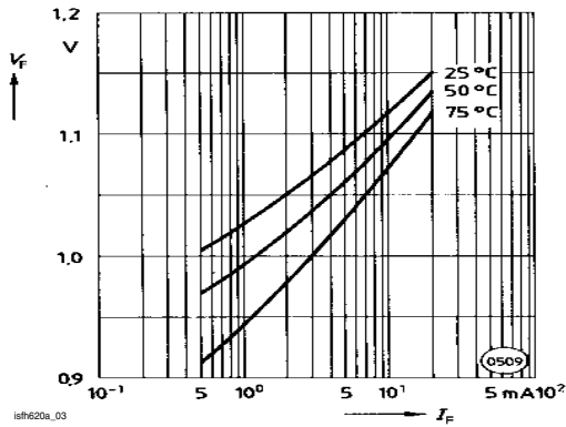
Fig. 4 Diode Forward Voltage (typ.) vs. Forward Current
