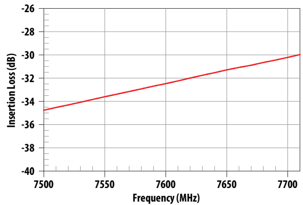
Figure 18. Tx-Ant Low Frequency Rejection, 7500 – 7710 MHz.
