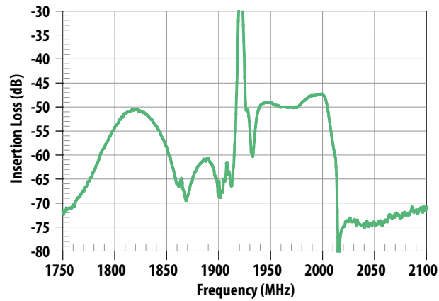
Figure 5. PCS Tx-Rx Isolation.
