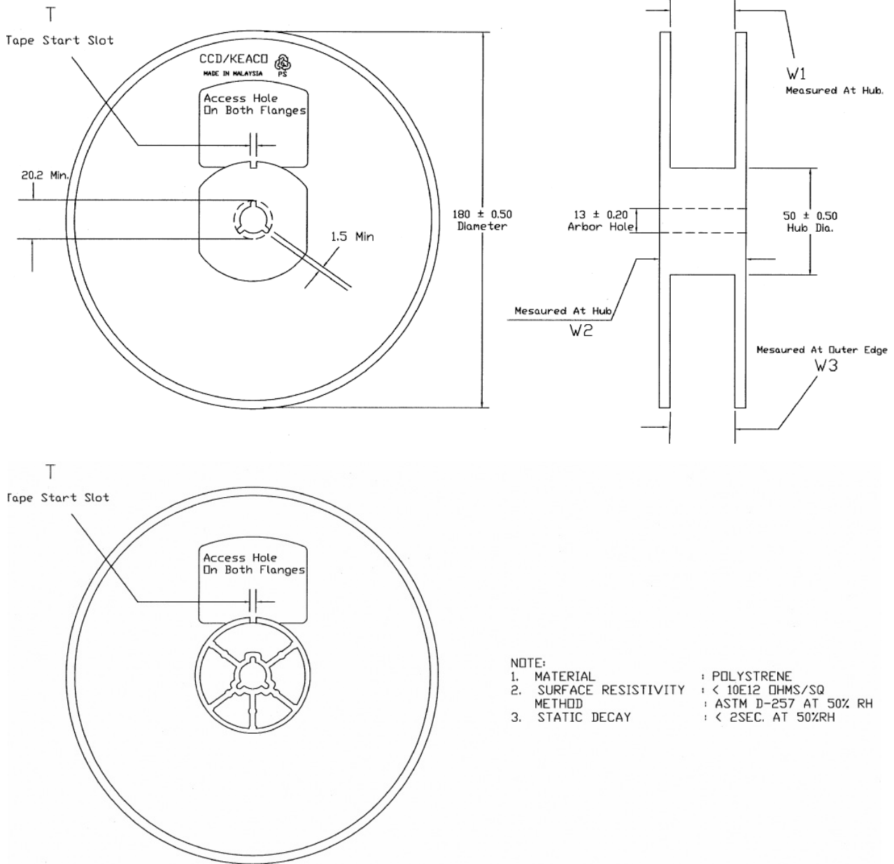
Figure 43. Reel Drawing
