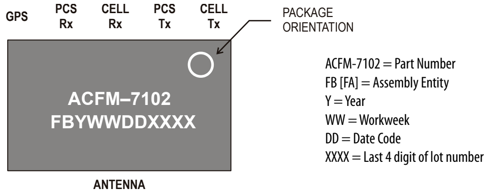
Figure 39. Package Marking.
