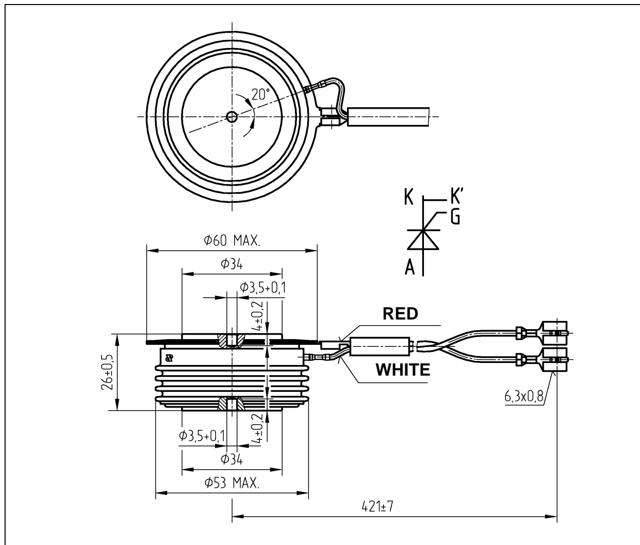
Fig. 10 Device Outline Drawing.
