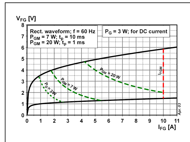
Fig. 9 Max. peak gate power loss.
