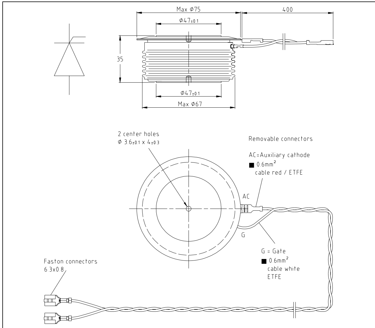
Fig. 12 Device Outline Drawing.
