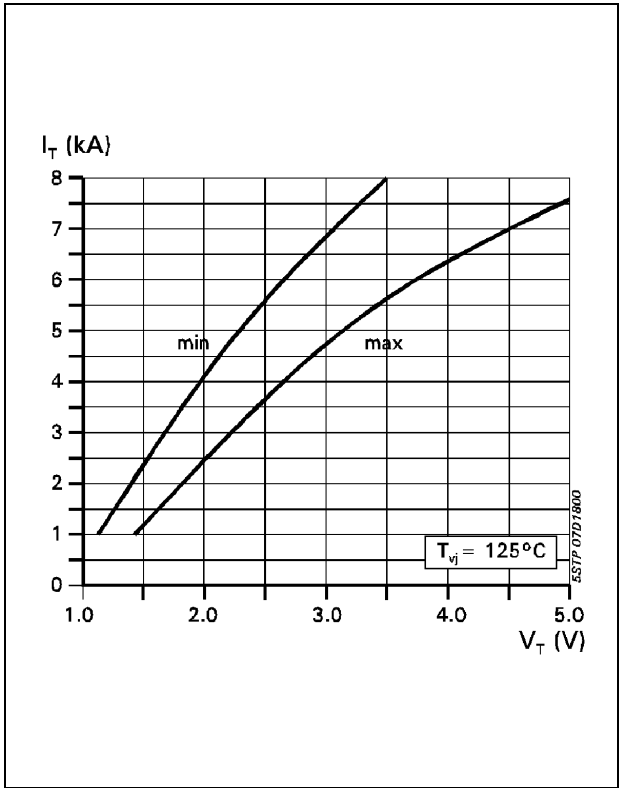
Fig. 3 On-state characteristics. T vj =125°C, 10ms half sine
