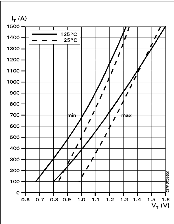
Fig. 2 On-state characteristics.
