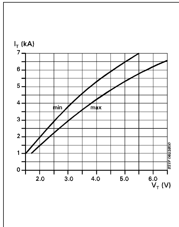
Fig. 3 On-state characteristics. T_j=125^\circ\text{C} , 10ms half sine
