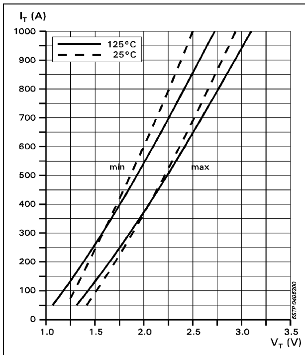
Fig. 2 On-state characteristics.
