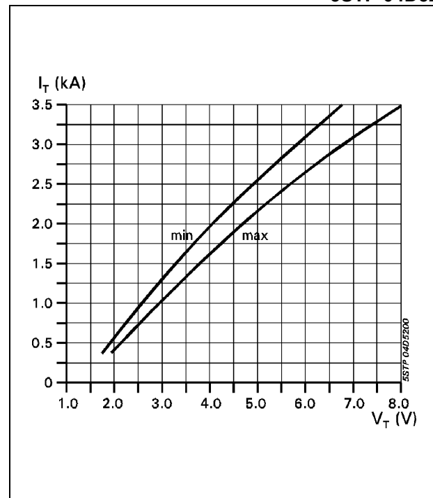
Fig. 3 On-state characteristics. T_J=125^\circ\text{C} , 10ms half sine
