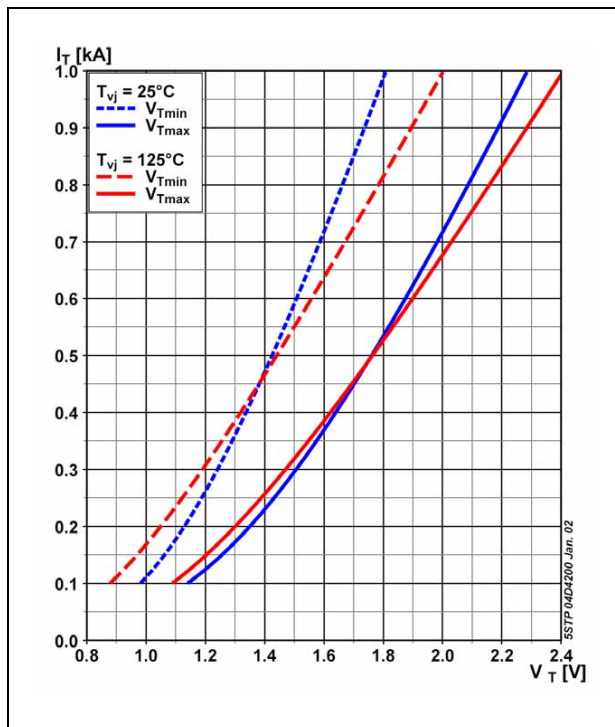
Fig. 2 On-state characteristics.
