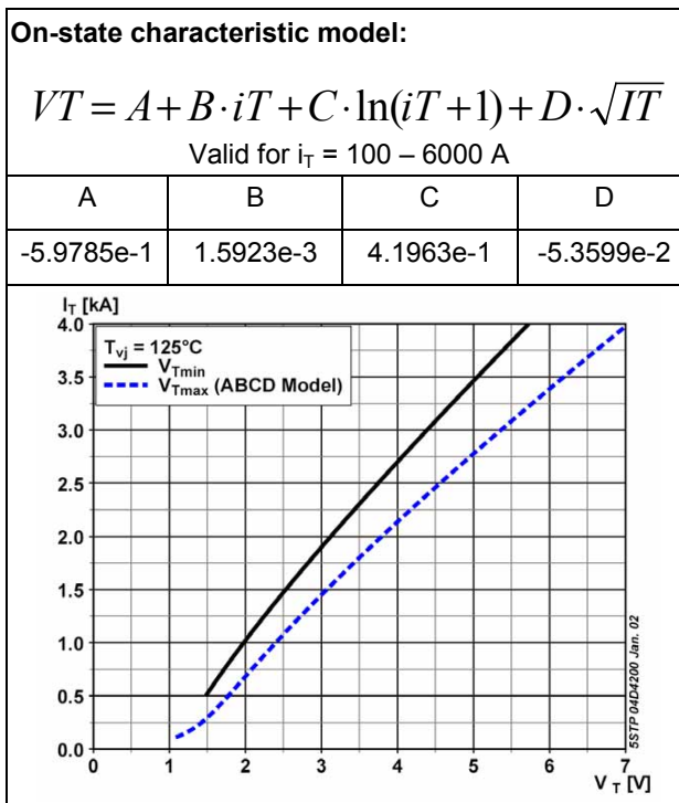
Fig. 3 On-state characteristics. T_{vj} = 125^\circ\text{C} , 10ms half sine
