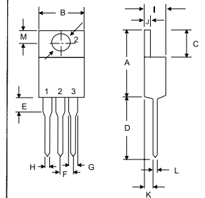
TO-220AB
