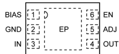
6-pin 2mm x 2mm MLF ® - Adjustable (ML)
