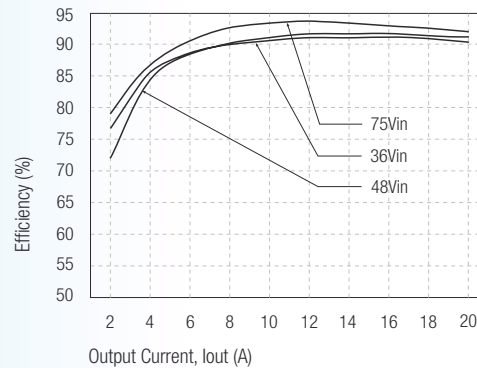
Input With Heatsink (7G-0022) RP100-4805SB
