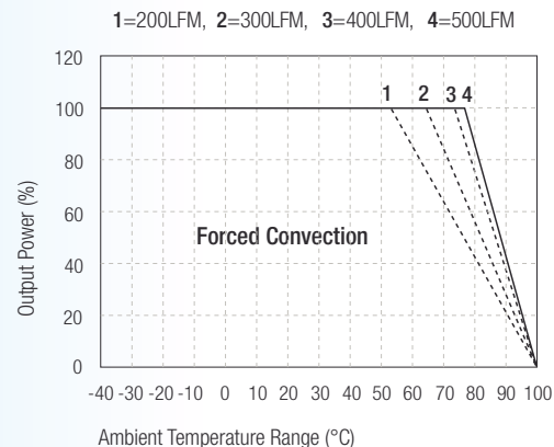
Input With Heatsink (7G-0022) RP100-4805SB
