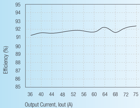
Input Without Heatsink RP100-4805SB
