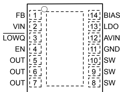
14- Pin 3mm x 3.5mm MLF® (HL)
