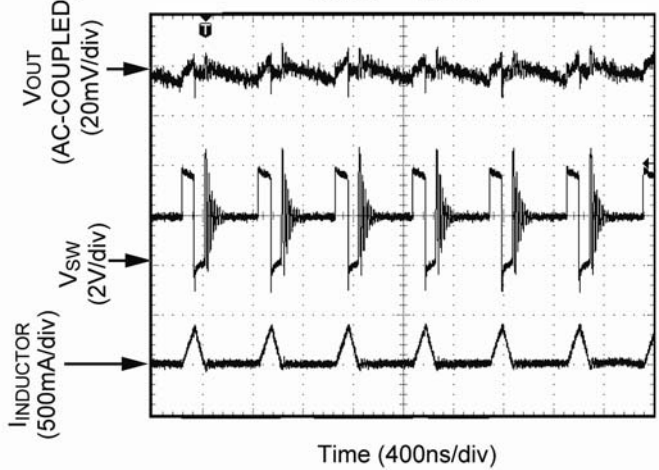
Switching Waveform – Continuous Mode I OUT = 300mA
