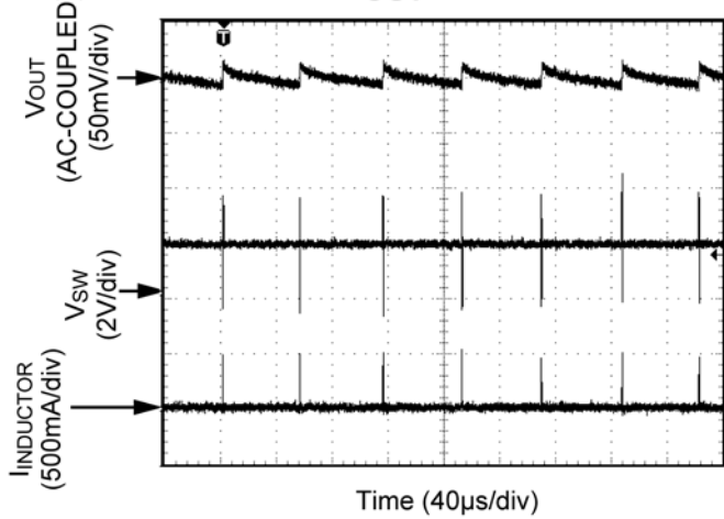
Switching Waveform – Discontinuous Mode I OUT = 50mA
