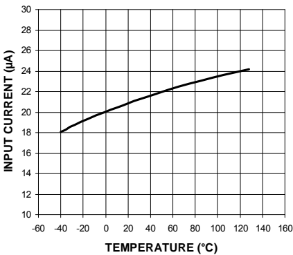
Quiescent Current vs. Temperature (Not Switching)
