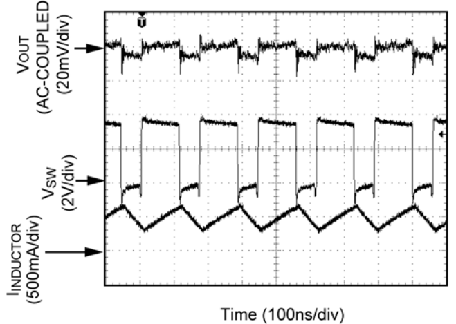
Switching Waveform – Continuous Mode I OUT = 400mA
