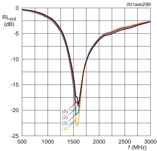
V_{CC} = 1.8 \text{ V}; P_i = -45 \text{ dBm}. (1) T_{\text{amb}} = -40 \text{ }^\circ\text{C} (2) T_{\text{amb}} = +25 \text{ }^\circ\text{C} (3) T_{\text{amb}} = +85 \text{ }^\circ\text{C} (4) T_{\text{amb}} = +125 \text{ }^\circ\text{C}
