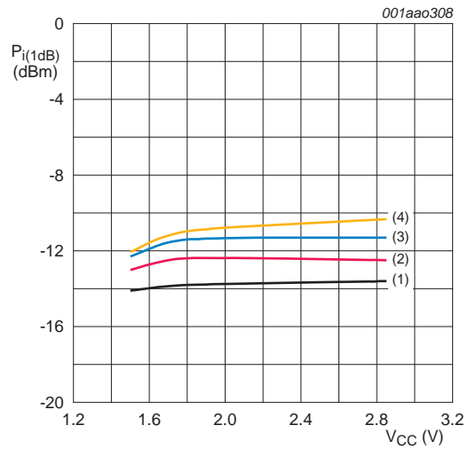
f = 1850 \text{ MHz} . (1) T_{\text{amb}} = -40 \text{ }^\circ\text{C} (2) T_{\text{amb}} = +25 \text{ }^\circ\text{C} (3) T_{\text{amb}} = +85 \text{ }^\circ\text{C} (4) T_{\text{amb}} = +125 \text{ }^\circ\text{C}
