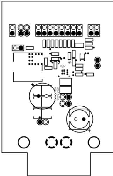
Figure 10. MIC26901 Evaluation Board Mid-Layer 1 (Ground Plane)
