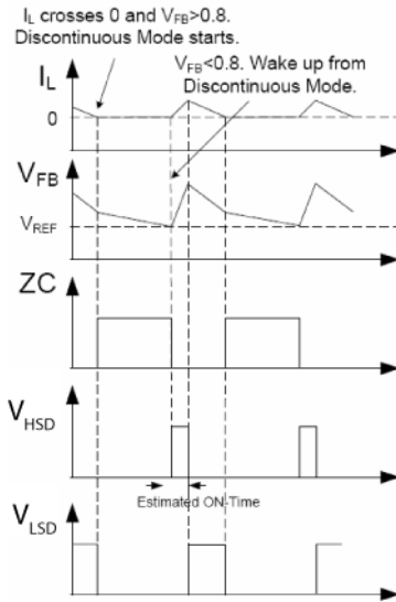
Figure 4. MIC26603 Control Loop Timing (Discontinuous Mode)
