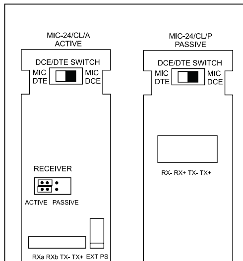
Figure 4. Strapping Diagram
