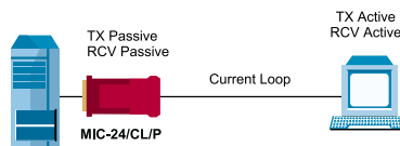
Figure 3. MIC-24/CL/P Passive Unit
