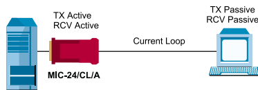
Figure 2. MIC-24/CL/A Active Unit with Active Receive
