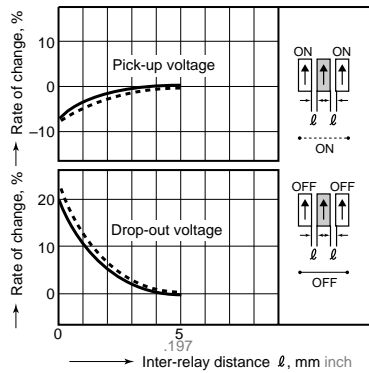
13-(2). Influence of adjacent mounting
