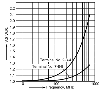
Tested sample: TN2-xxV V.S.W.R.
