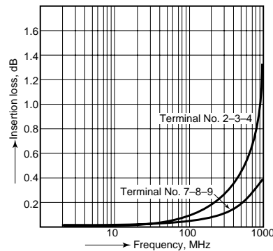
Tested sample: TN2-xxV Insertion loss characteristics
