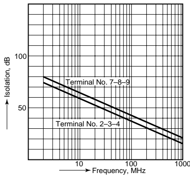
Tested sample: TN2-xxV Isolation characteristics
