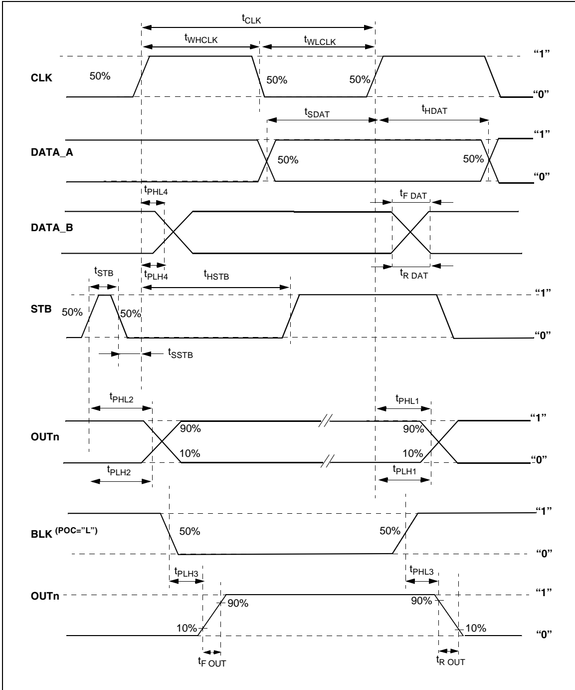
Figure 5. AC characteristics waveform
