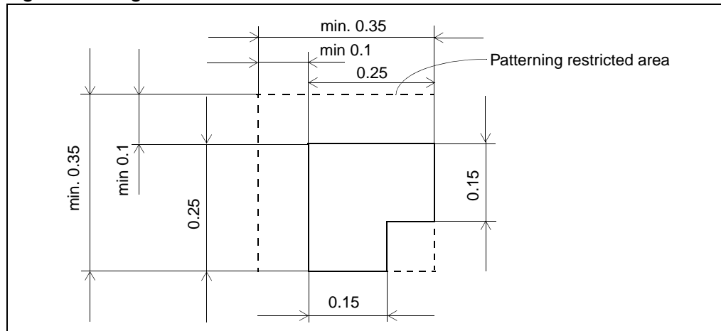
Figure 4. Alignment marks
