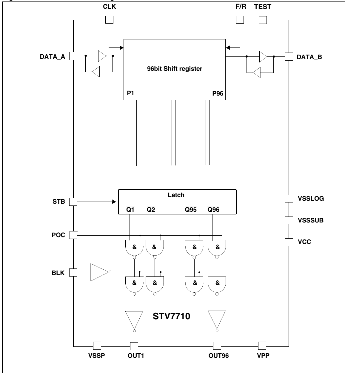
Figure 2. STV7710 block diagram
