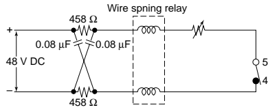
Circuit
