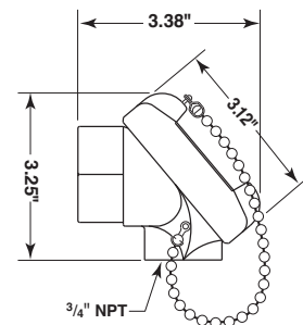
Junction box available with SPST or SPDT reed switch
