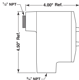
Junction box supplied with DPDT relay
