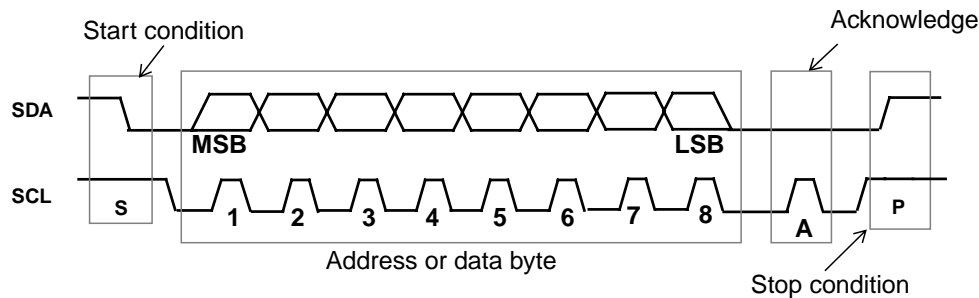
Figure 35 : Serial Interface Data Transfer Protocol
