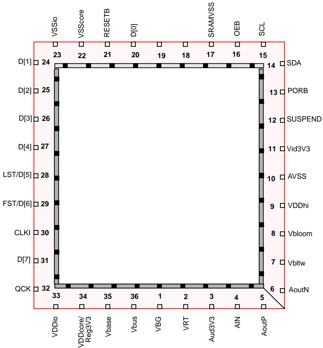
Figure 55 : 36 pin CLCC package pin assignment
