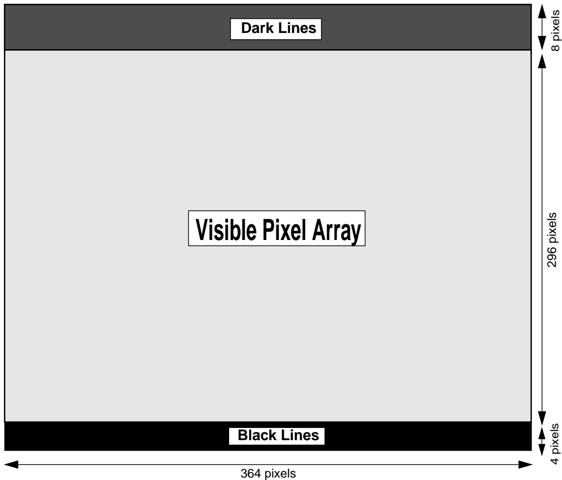
Figure 11 : Physical position of Black and Dark Lines
