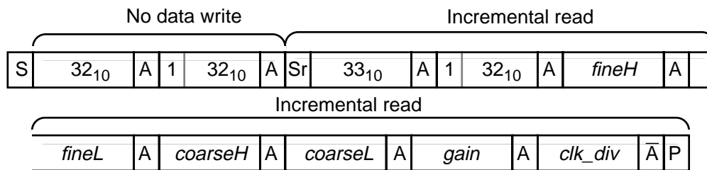
Figure 44 : Multiple location read.
