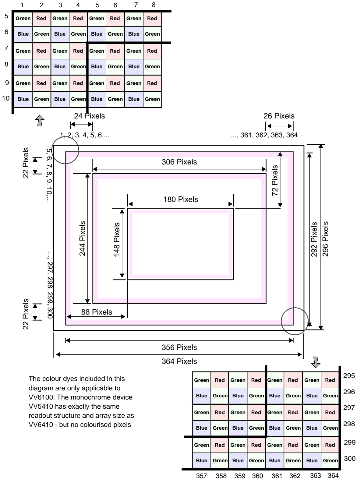
Figure 3 : Image Readout Formats
