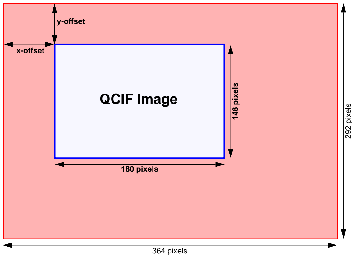
Figure 9 : Pan/Tilt QCIF Image Format
