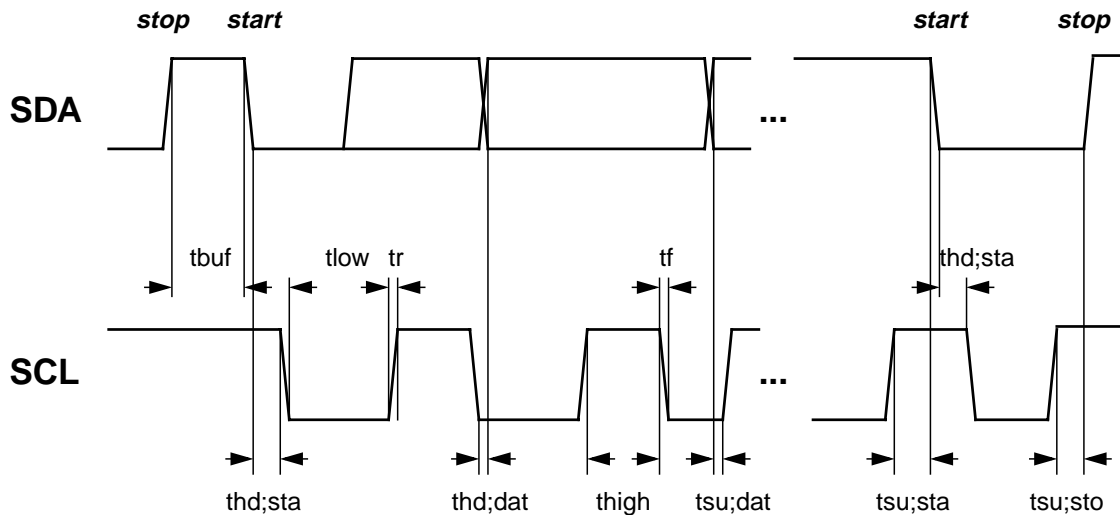
Figure 45 : Serial Interface Timing Characteristics
