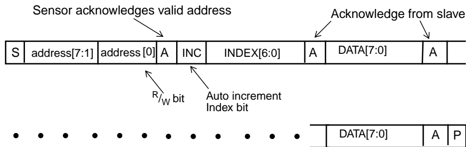
Figure 37 : Serial Interface Data Format
