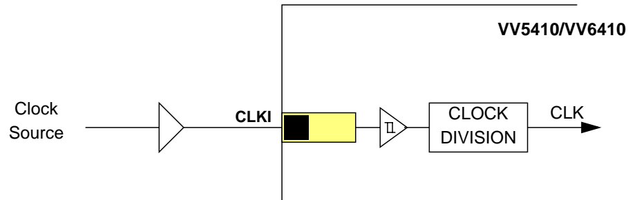
Figure 46 : CMOS Clock Source
