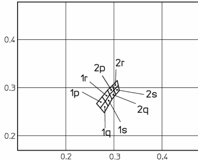
Chromaticity Coordinates Tolerance Each Rank: +/-0.01
