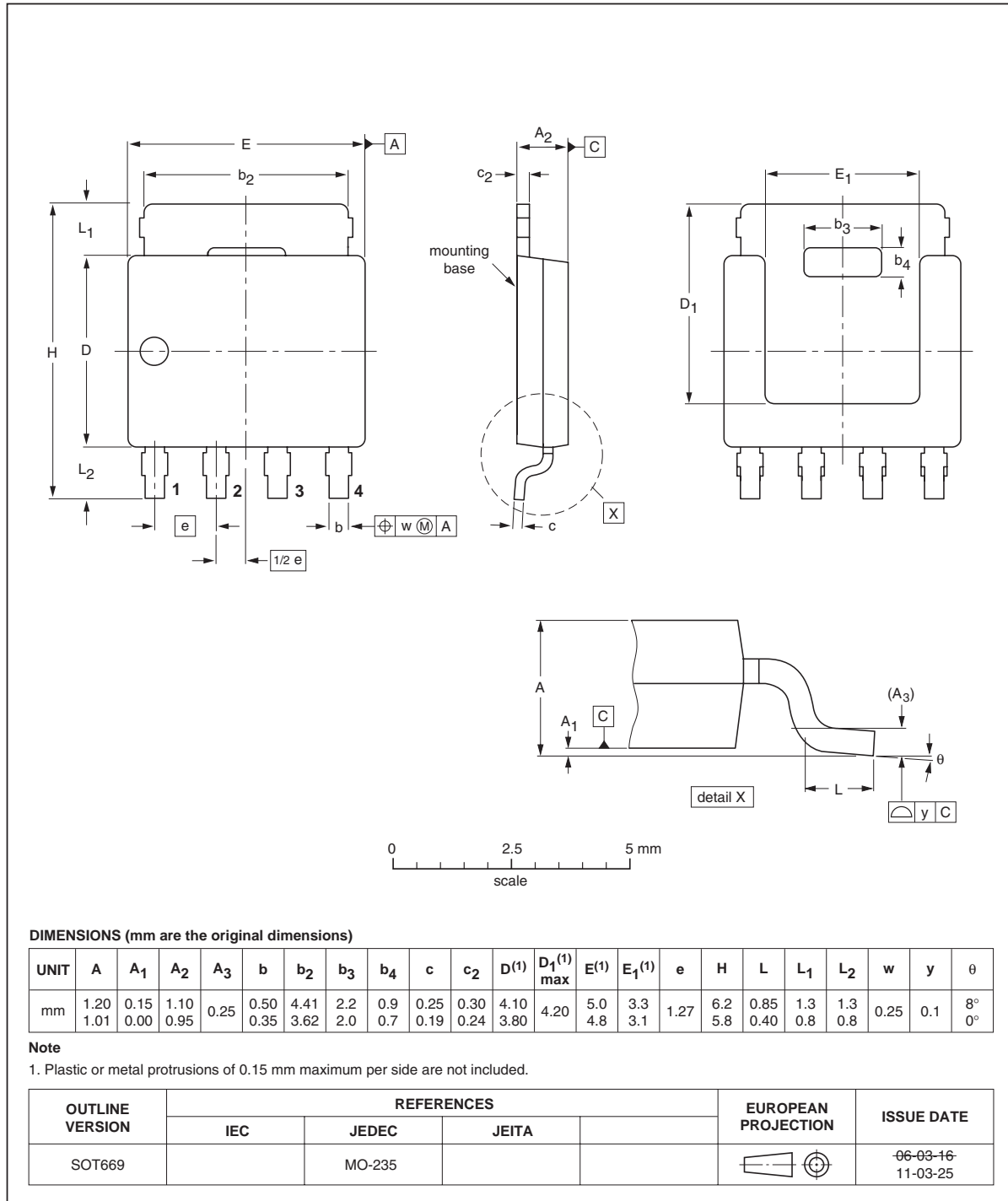
Fig 18. Package outline SOT669 (LFPAK; Power-SO8)
