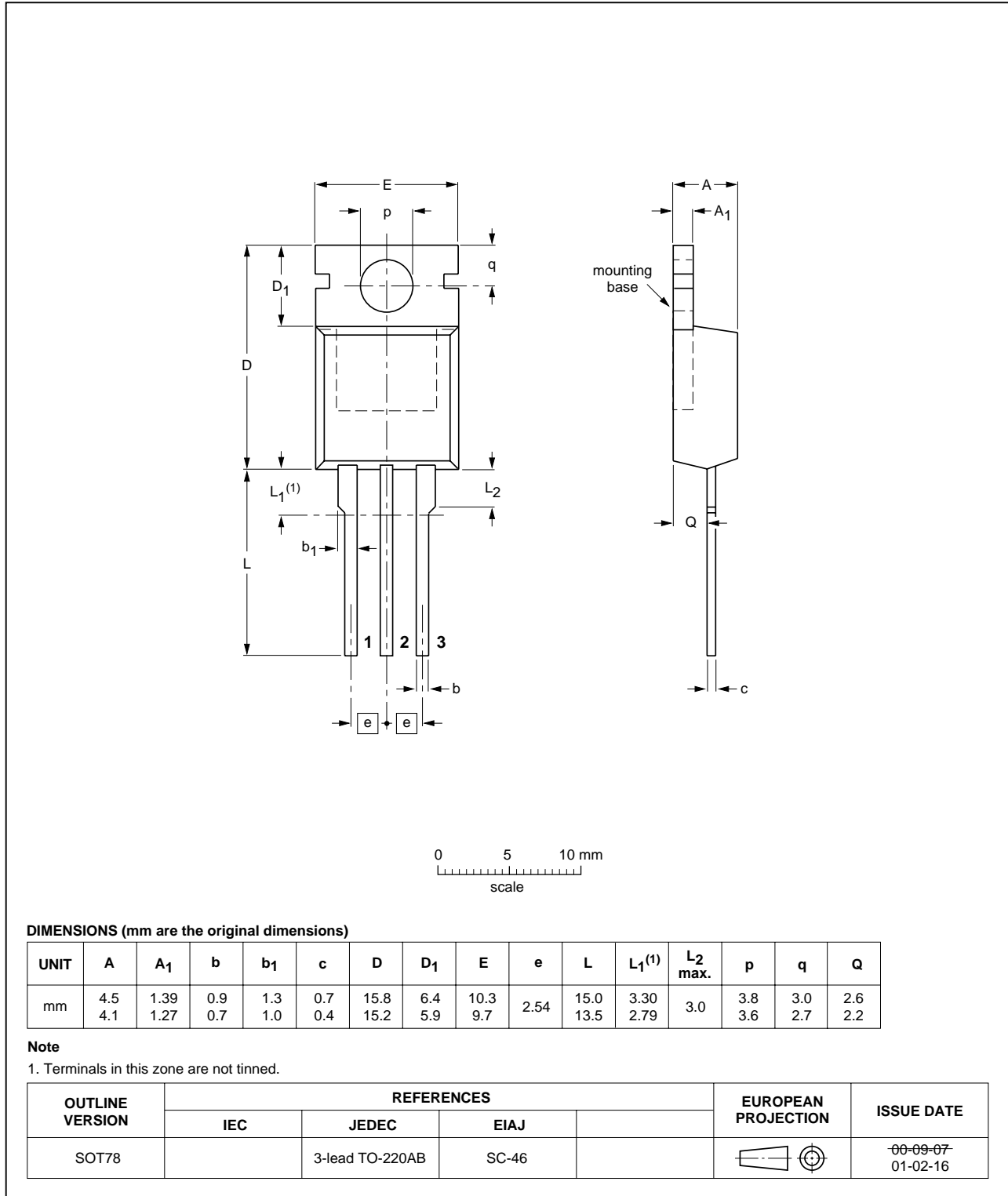
Fig 14. SOT78 (TO-220AB).
