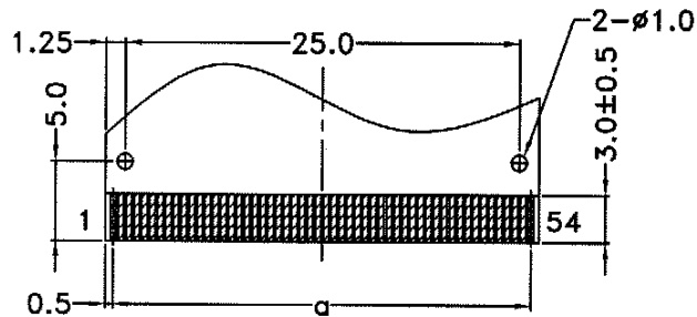
FPC Detail Scale:2/1
