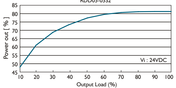
Efficiency Vs Output Load RDD05-05S2
