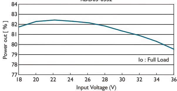
Efficiency Vs Input Voltage RDD05-05S2
