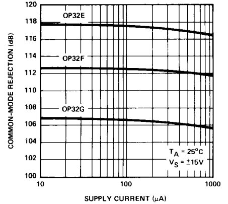
COMMON-MODE REJECTION vs SUPPLY CURRENT
