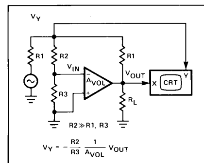
TEST CIRCUIT
