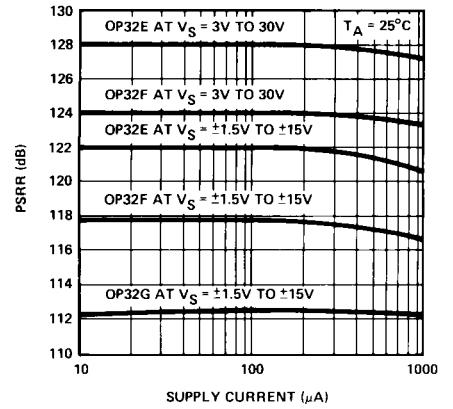
POWER SUPPLY REJECTION vs SUPPLY CURRENT
