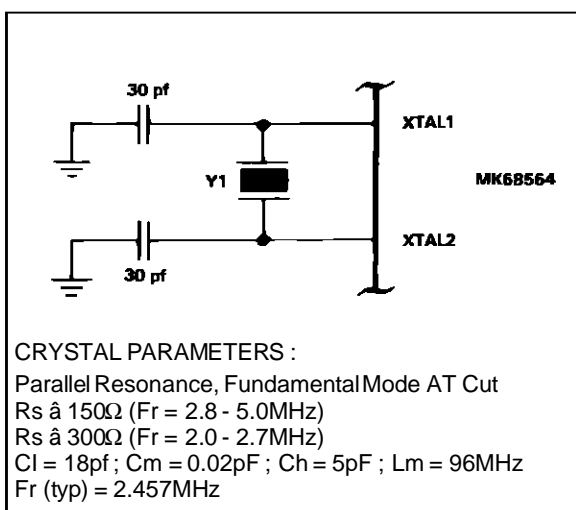
Figure 8 : SIO External Oscillator Components.
