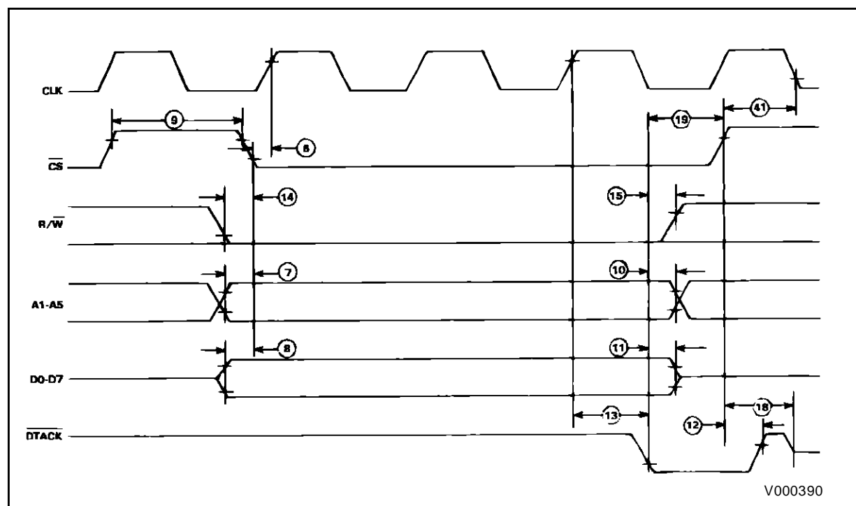
Figure 16 : Write Cycle.
