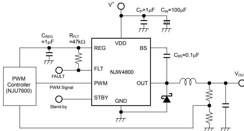
Synchronous PWM step down switching regulator
